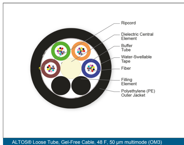
ALTOS® Loose Tube, Gel-Free Cable, 48 F, 50 µm multimode (OM3)
